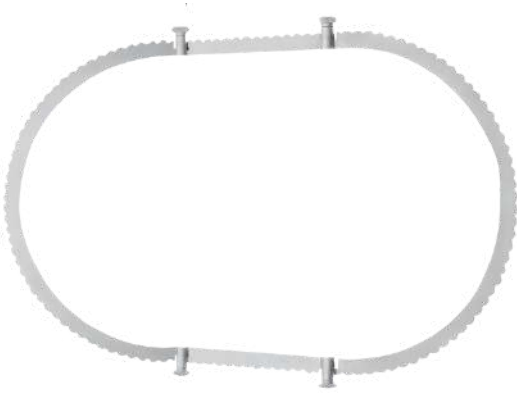
Ø 215 x 355 mm 10.509 Ø 265 x 495 mm 10.510 Ø 405 x 595 mm 10.511 Parçalı oval çember
